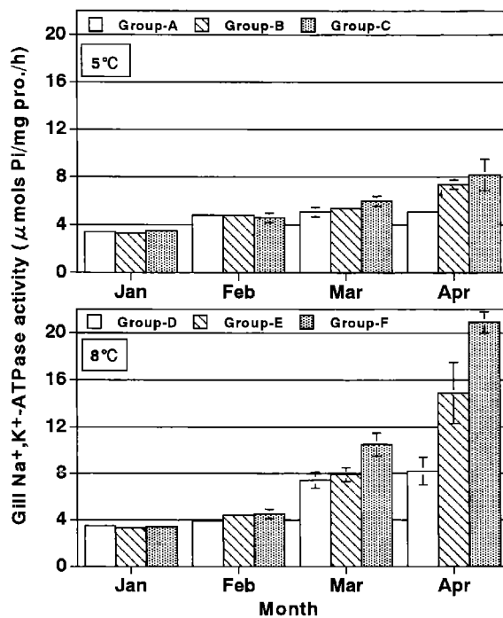
Fig. 3. Changes in gill \text{Na}^+, \text{K}^+ -ATPase activity in groups A-F of sockeye salmon reared in fresh water from January to April. Groups A, B and C were kept at 3-5°C (upper) and groups D, E and F were kept at 7-8°C (lower). Bars indicate SE.
