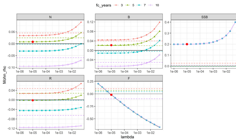
tuned VPA with ridge penalty
